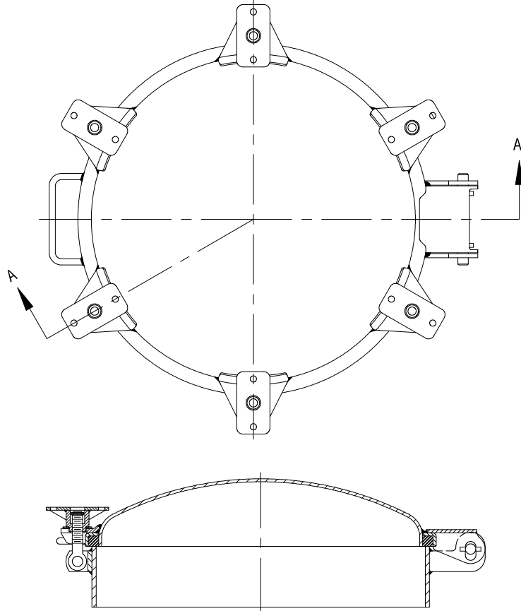
Section A-A Model 8355
