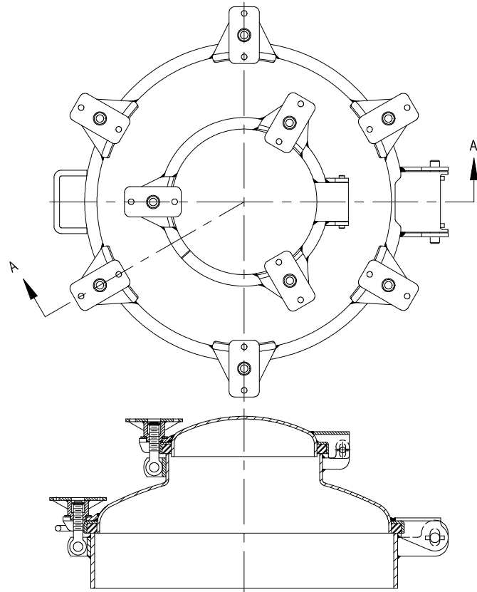
Section A-A Model 8387
